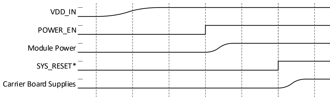
Figure 3: Power-up Sequence
